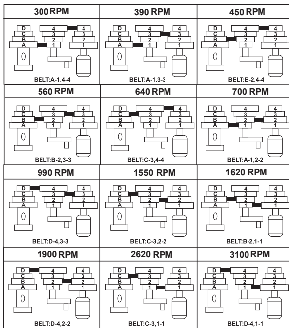
DRILLING SPEED TABLE (RPM)-FOR 15 IN. (381MM) DRILL PRESS
