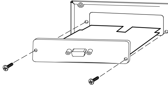
Figure 21. Removing the Single-Port Card
