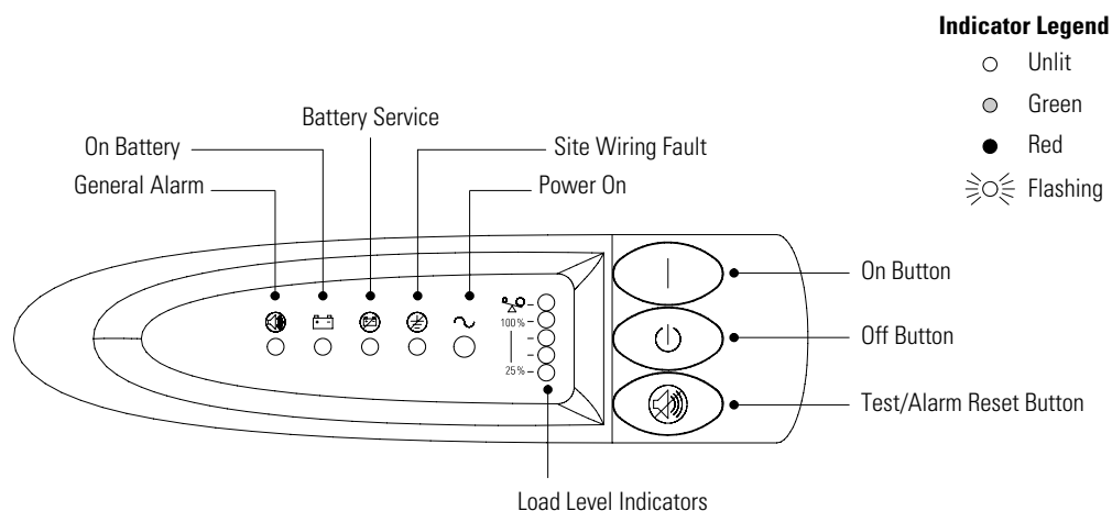
Figure 30. Alarm Indicators
