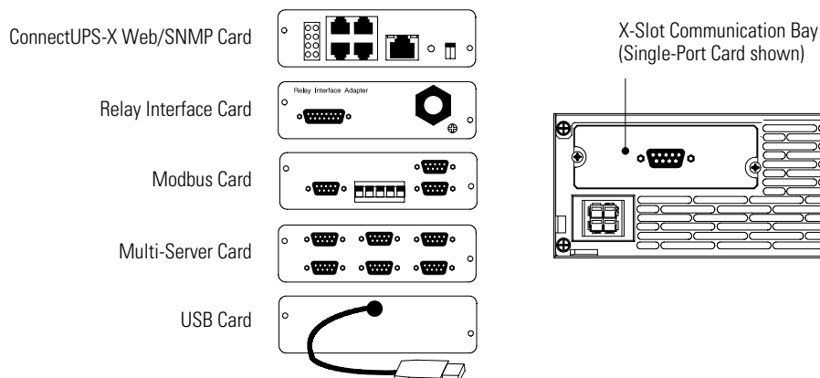
Figure 19. Optional X-Slot Cards
