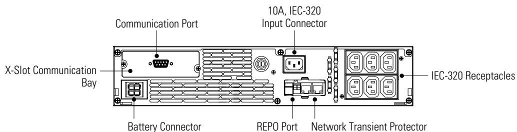
Figure 14. 1000/1500 VA, 230V Rear Panel
