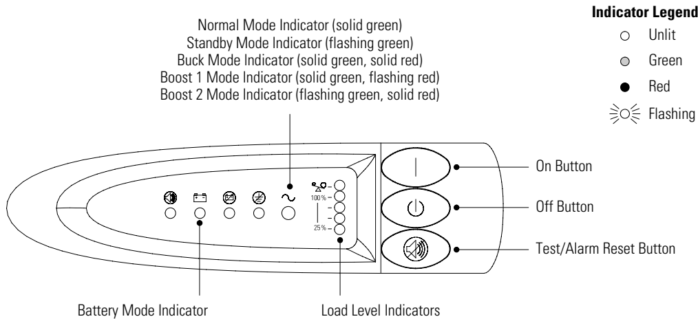
Figure 16. UPS Front Panel
