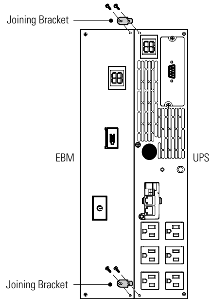
Figure 10. Installing the Joining Brackets
