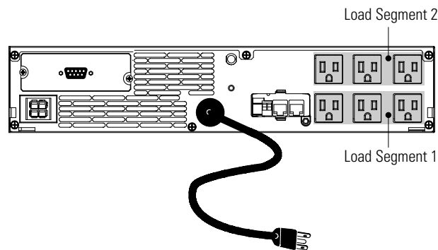
Figure 24. UPS Load Segments (Low Voltage Models)
