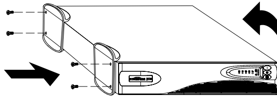
Figure 7. Installing the UPS Pedestals
