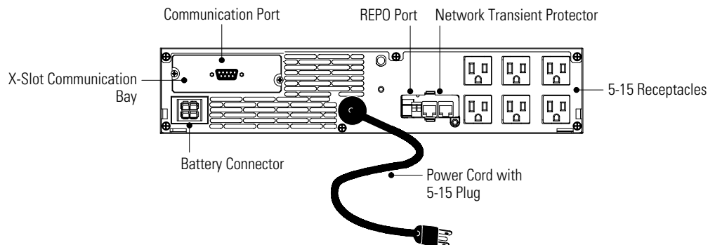
Figure 13. 1000/1500 VA, 120V and 1000 VA, 100V Rear Panel
