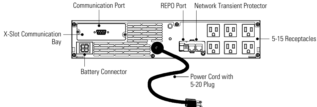
Figure 15. 1500 VA, 100V Rear Panel
